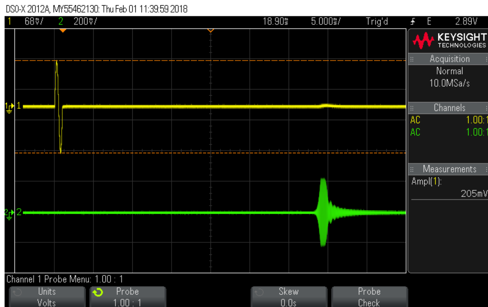
Figure 39: Transmit latency, USB-D1. Latency 34 ms.
