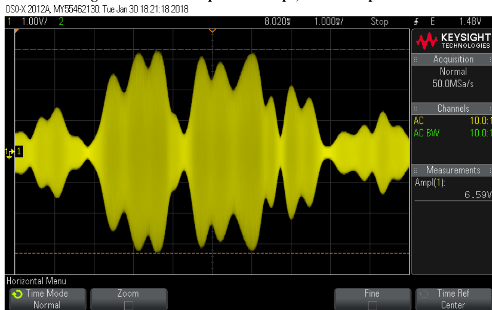
Figure 9: 100W PEP speech envelope, \approx 6 dB compression.
