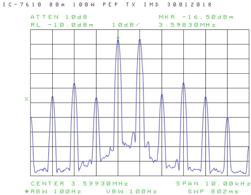
Figure 12: Spectral display of 2-tone IMD at 3.6 MHz, 100W PEP.
